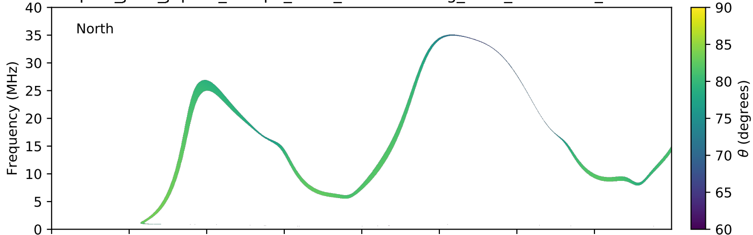
expres_juno_jupiter_europa_isaac_lossc-wid1deg_3kev_20180619_v01.cdf
