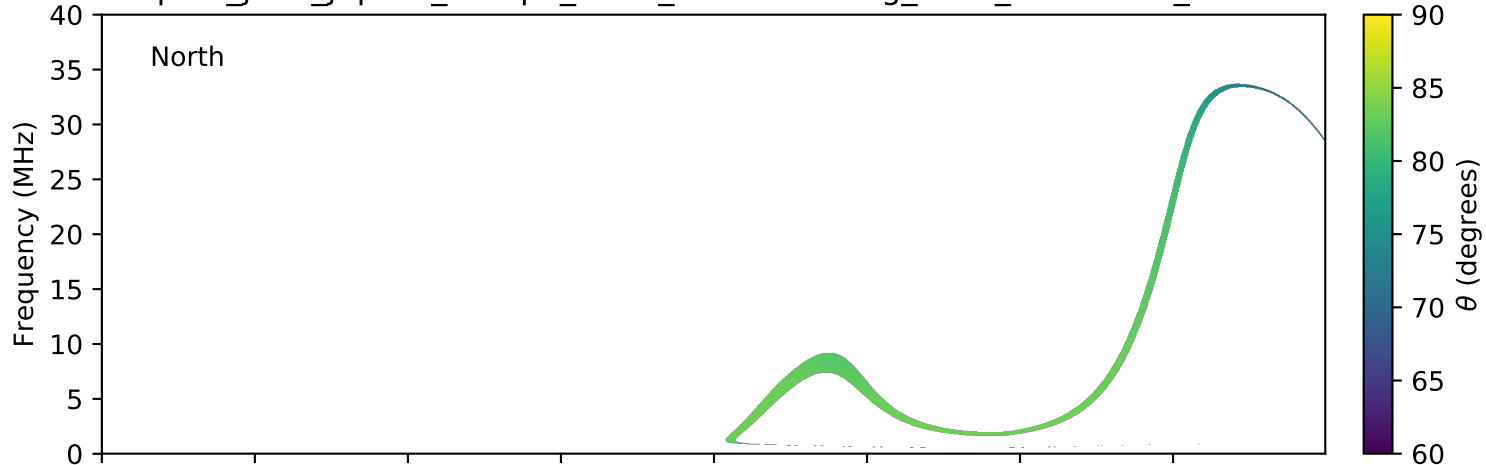
expres_juno_jupiter_europa_isaac_lossc-wid1deg_3kev_20180615_v01.cdf
