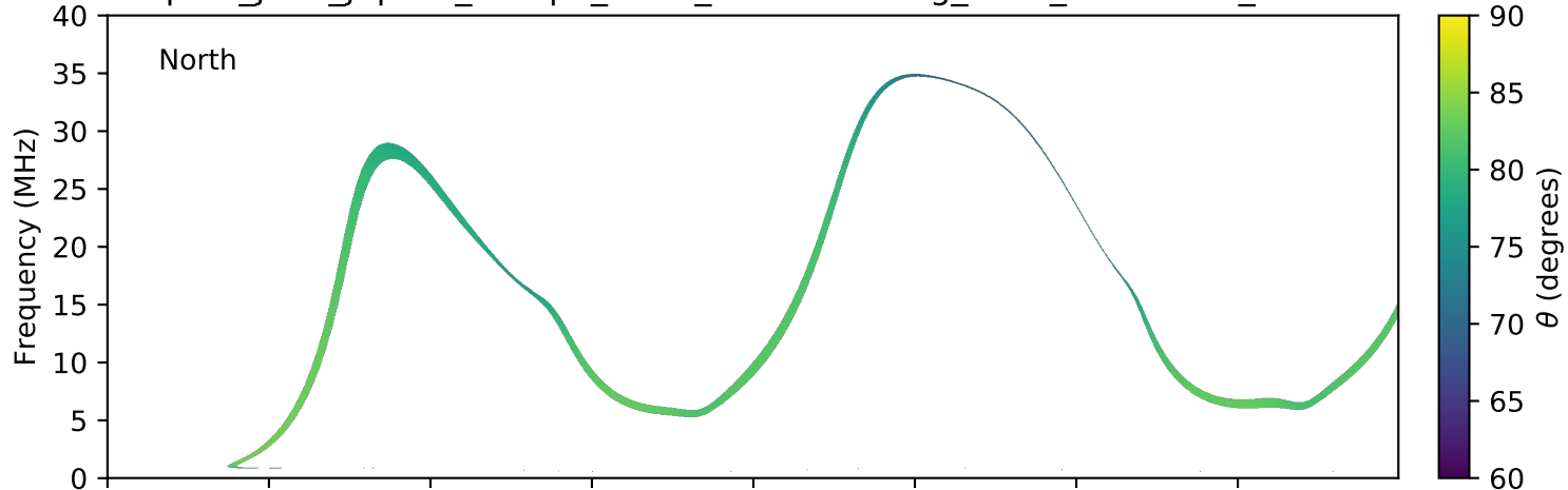
expres_juno_jupiter_europa_isaac_lossc-wid1deg_3kev_20180612_v01.cdf
