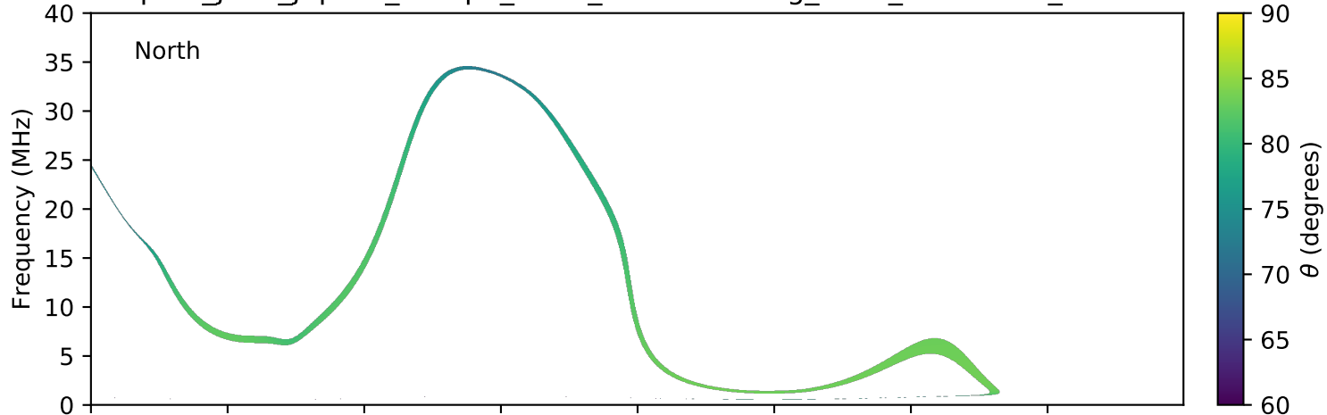
expres_juno_jupiter_europa_isaac_lossc-wid1deg_3kev_20180609_v01.cdf
