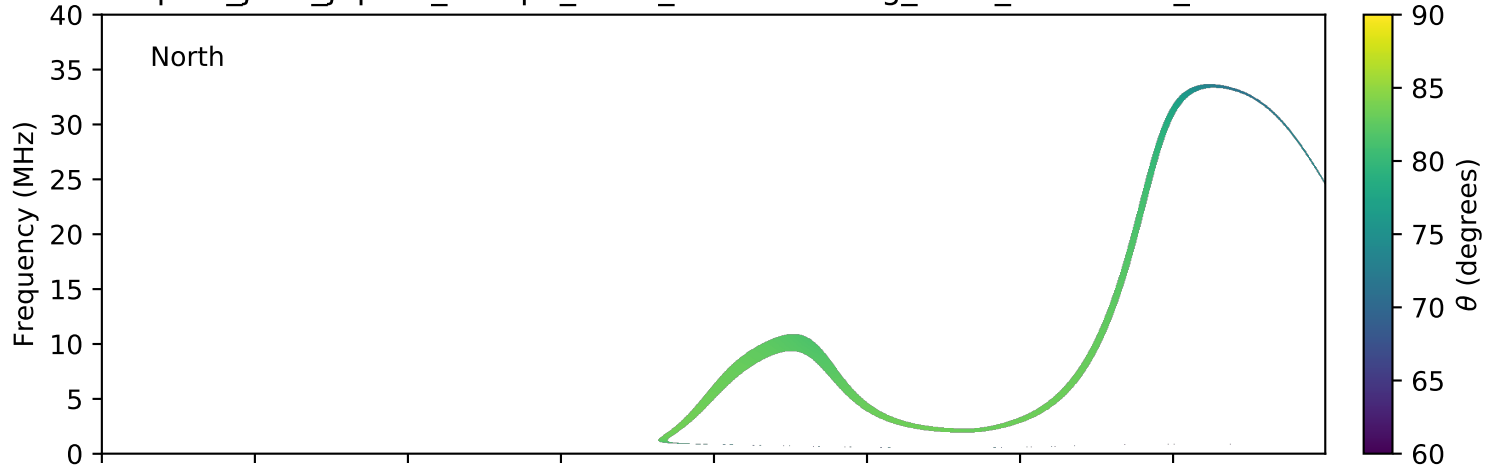
expres_juno_jupiter_europa_isaac_lossc-wid1deg_3kev_20180608_v01.cdf
