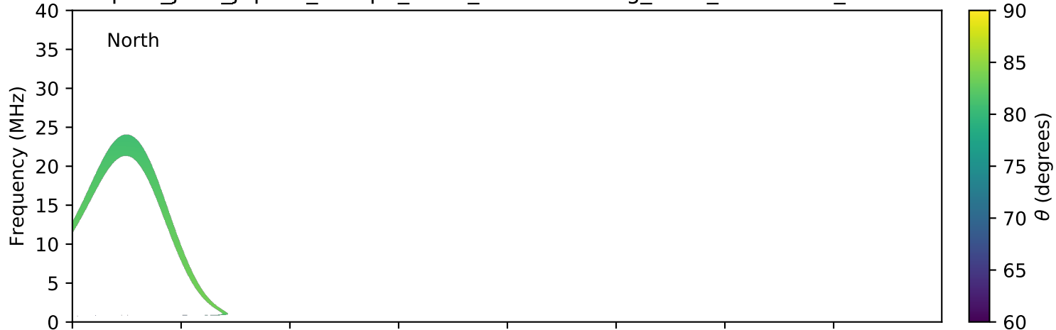
expres_juno_jupiter_europa_isaac_lossc-wid1deg_3kev_20180606_v01.cdf
