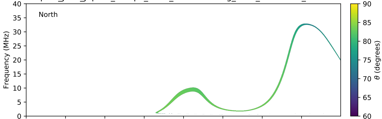
expres_juno_jupiter_europa_isaac_lossc-wid1deg_3kev_20180601_v01.cdf
