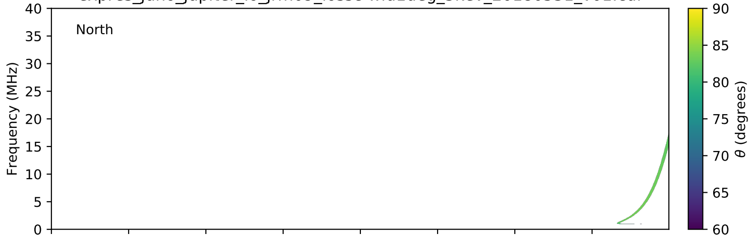
expres_juno_jupiter_io_jrm09_lossc-wid1deg_3kev_20180531_v01.cdf
