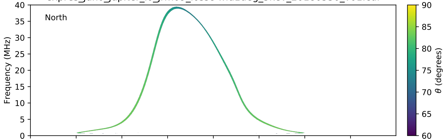
expres_juno_jupiter_io_jrm09_lossc-wid1deg_3kev_20180530_v01.cdf
