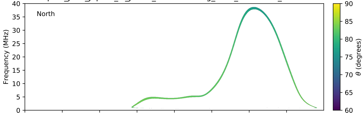
expres_juno_jupiter_io_jrm09_lossc-wid1deg_3kev_20180528_v01.cdf
