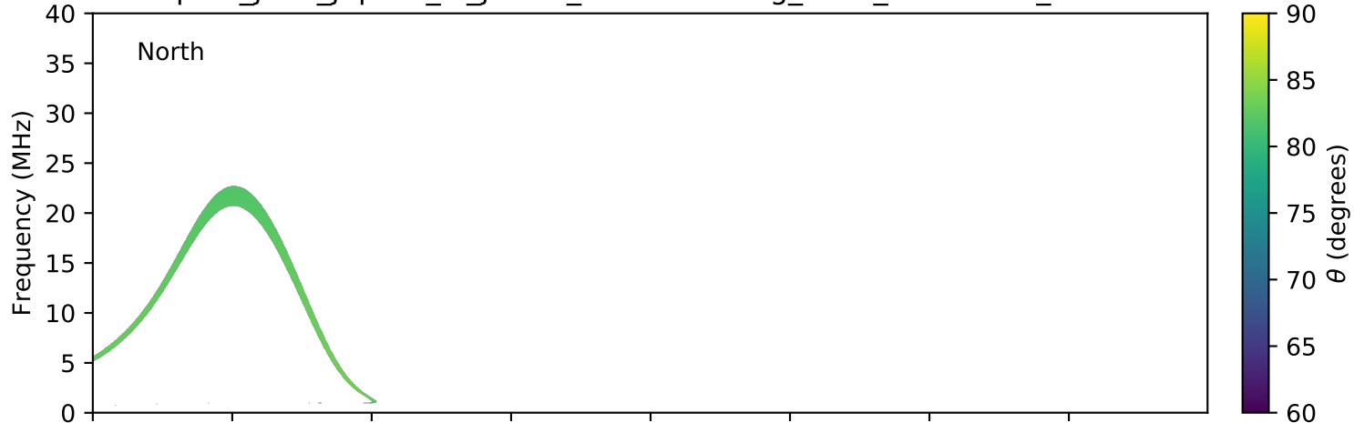
expres_juno_jupiter_io_jrm09_lossc-wid1deg_3kev_20180527_v01.cdf
