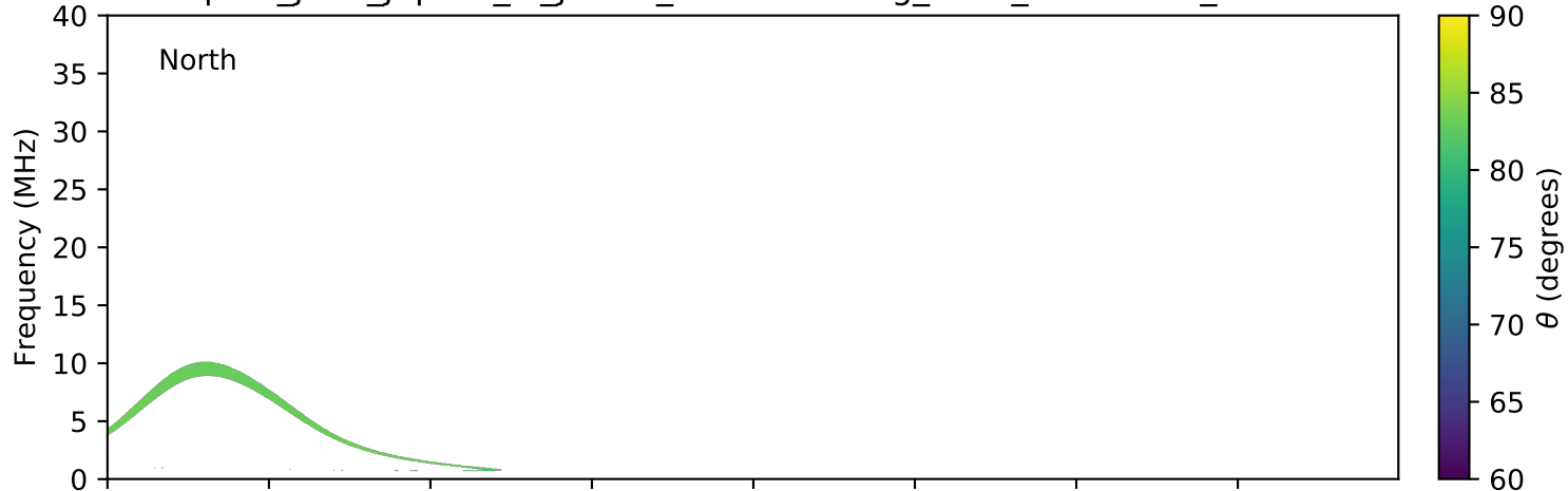
expres_juno_jupiter_io_jrm09_lossc-wid1deg_3kev_20180525_v01.cdf
