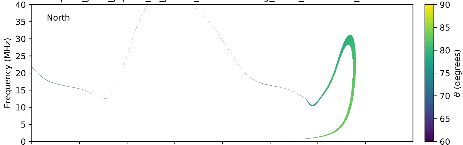
expres_juno_jupiter_io_jrm09_lossc-wid1deg_3kev_20180523_v01.cdf
