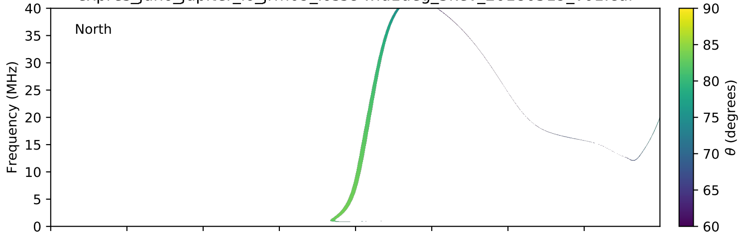
expres_juno_jupiter_io_jrm09_lossc-wid1deg_3kev_20180519_v01.cdf
