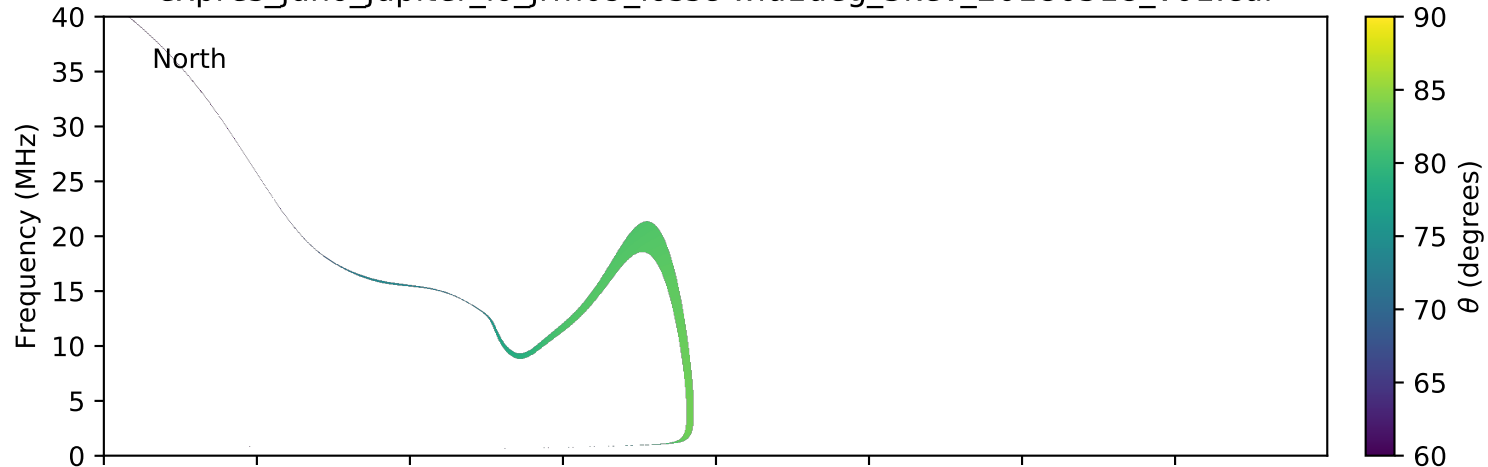
expres_juno_jupiter_io_jrm09_lossc-wid1deg_3kev_20180518_v01.cdf
