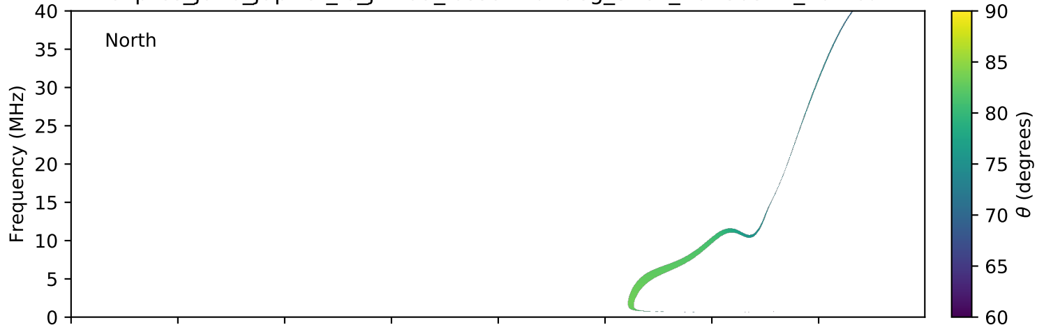
expres_juno_jupiter_io_jrm09_lossc-wid1deg_3kev_20180517_v01.cdf
