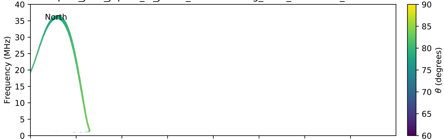
expres_juno_jupiter_io_jrm09_lossc-wid1deg_3kev_20180513_v01.cdf
