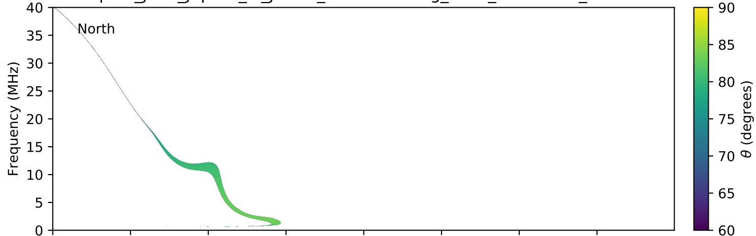
expres_juno_jupiter_io_jrm09_lossc-wid1deg_3kev_20180511_v01.cdf
