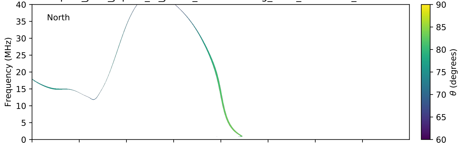
expres_juno_jupiter_io_jrm09_lossc-wid1deg_3kev_20180509_v01.cdf
