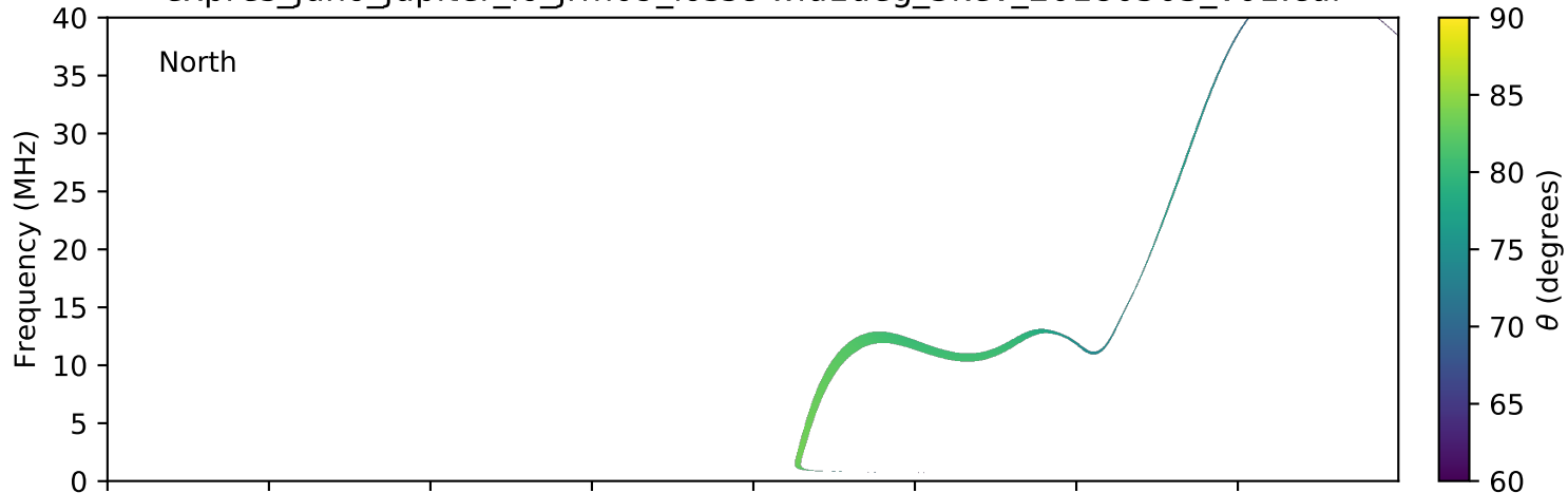
expres_juno_jupiter_io_jrm09_lossc-wid1deg_3kev_20180503_v01.cdf
