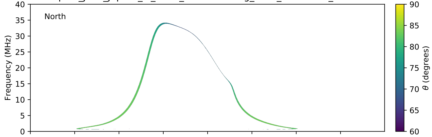
expres_juno_jupiter_io_isaac_lossc-wid1deg_3kev_20180530_v01.cdf
