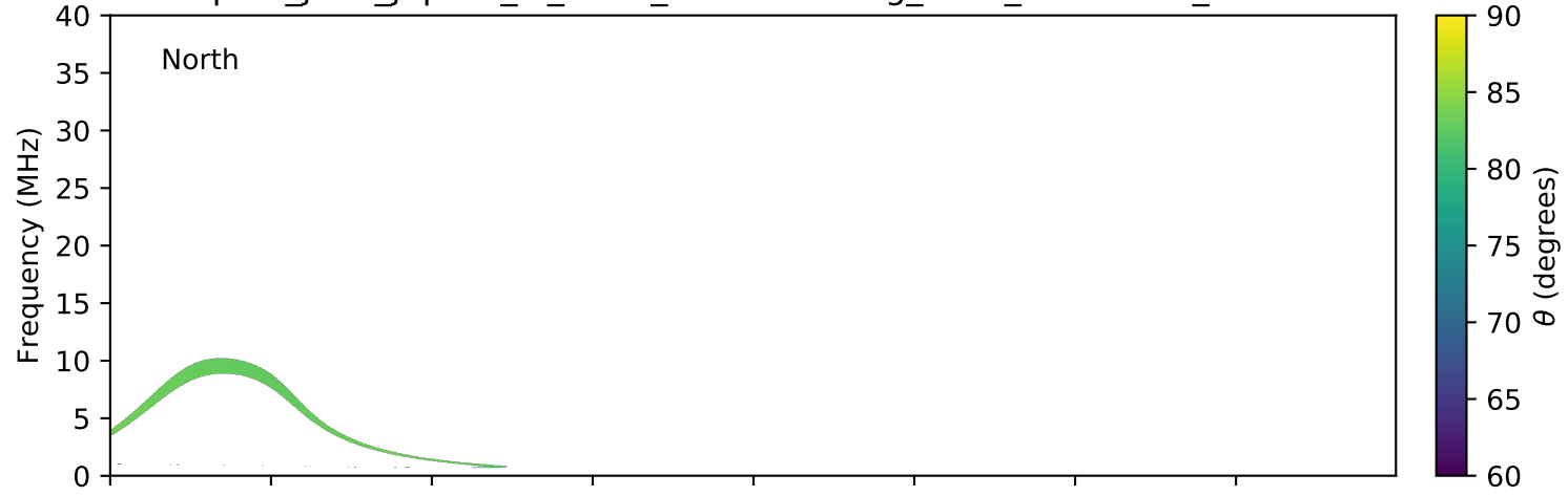
expres_juno_jupiter_io_isaac_lossc-wid1deg_3kev_20180525_v01.cdf
