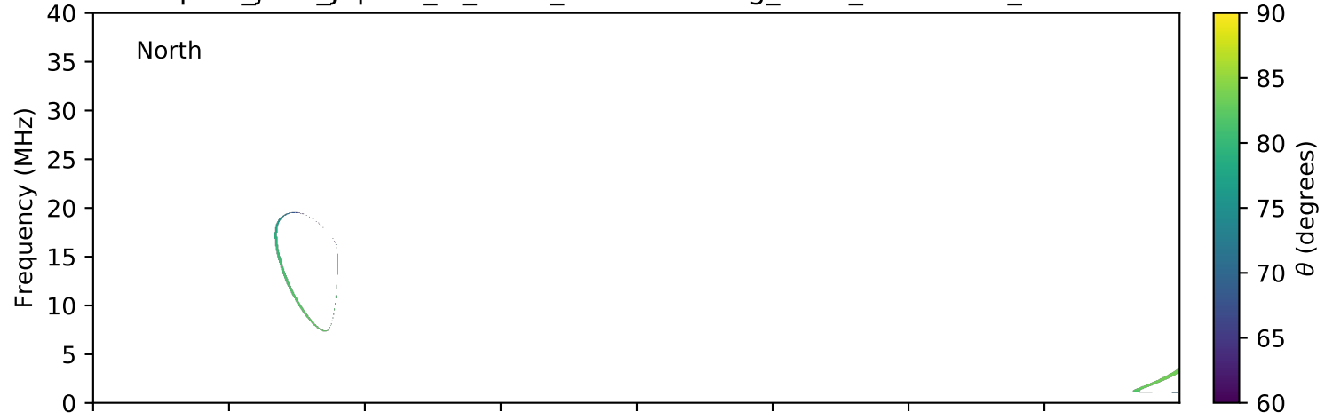
expres_juno_jupiter_io_isaac_lossc-wid1deg_3kev_20180524_v01.cdf
