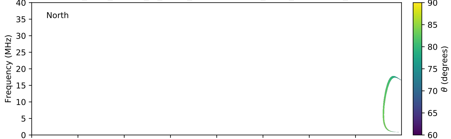
expres_juno_jupiter_io_isaac_lossc-wid1deg_3kev_20180522_v01.cdf
