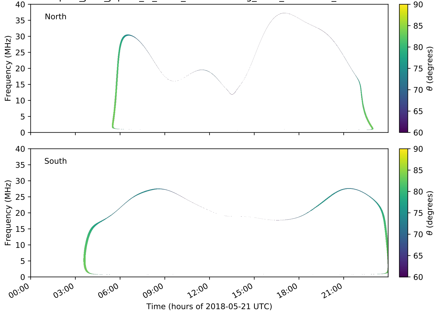
expres_juno_jupiter_io_isaac_lossc-wid1deg_3kev_20180521_v01.cdf
