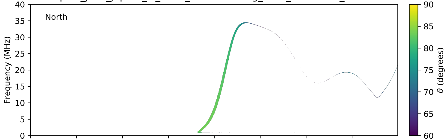
expres_juno_jupiter_io_isaac_lossc-wid1deg_3kev_20180519_v01.cdf
