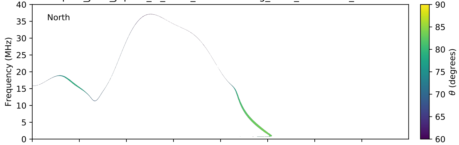
expres_juno_jupiter_io_isaac_lossc-wid1deg_3kev_20180516_v01.cdf
