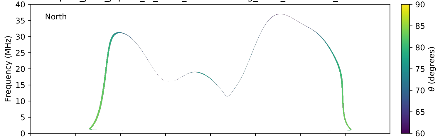
expres_juno_jupiter_io_isaac_lossc-wid1deg_3kev_20180514_v01.cdf
