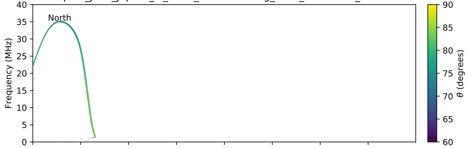
expres_juno_jupiter_io_isaac_lossc-wid1deg_3kev_20180513_v01.cdf
