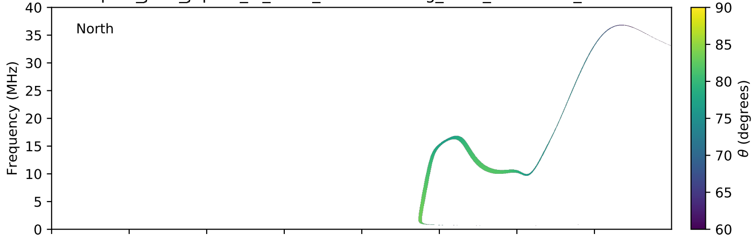
expres_juno_jupiter_io_isaac_lossc-wid1deg_3kev_20180510_v01.cdf
