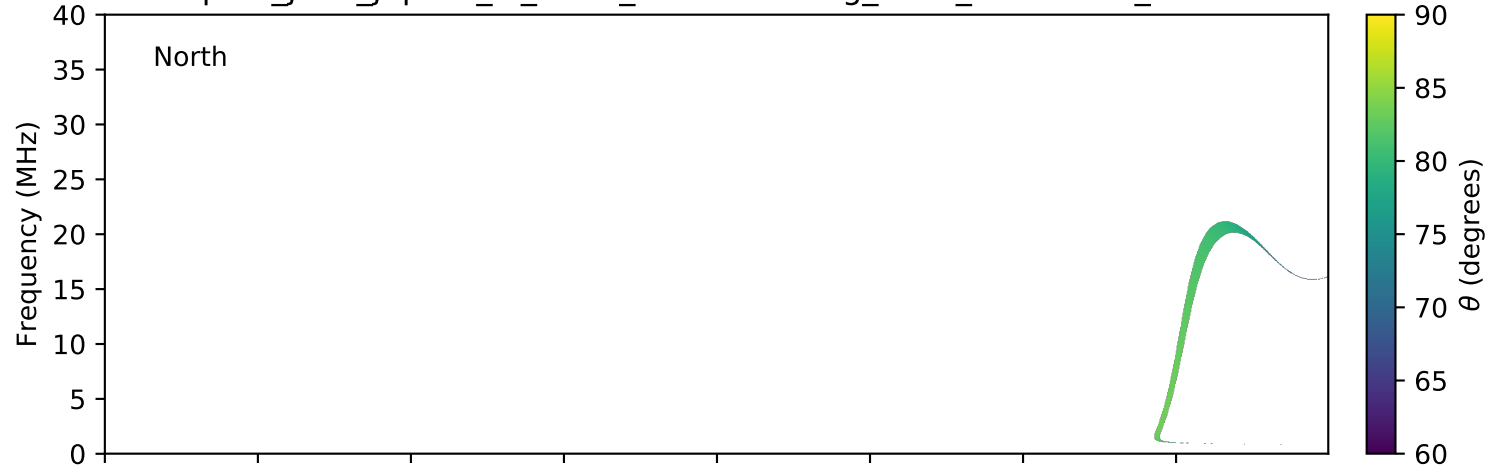
expres_juno_jupiter_io_isaac_lossc-wid1deg_3kev_20180508_v01.cdf
