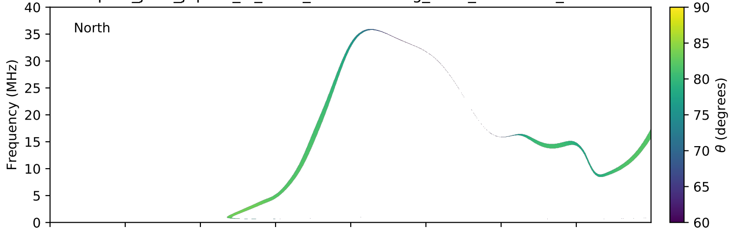
expres_juno_jupiter_io_isaac_lossc-wid1deg_3kev_20180505_v01.cdf
