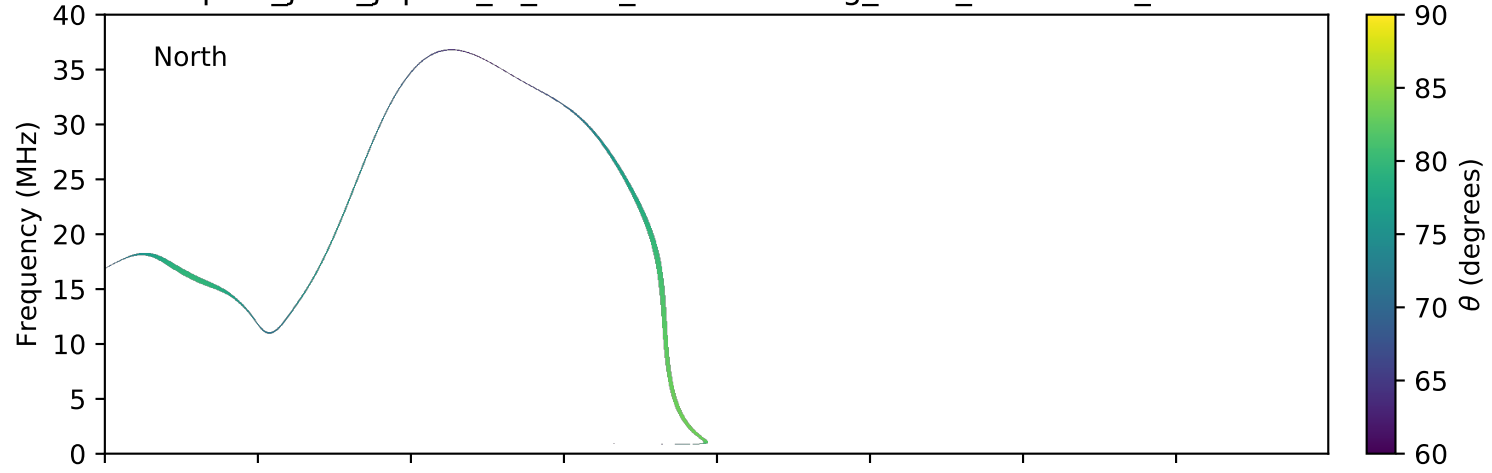
expres_juno_jupiter_io_isaac_lossc-wid1deg_3kev_20180502_v01.cdf
