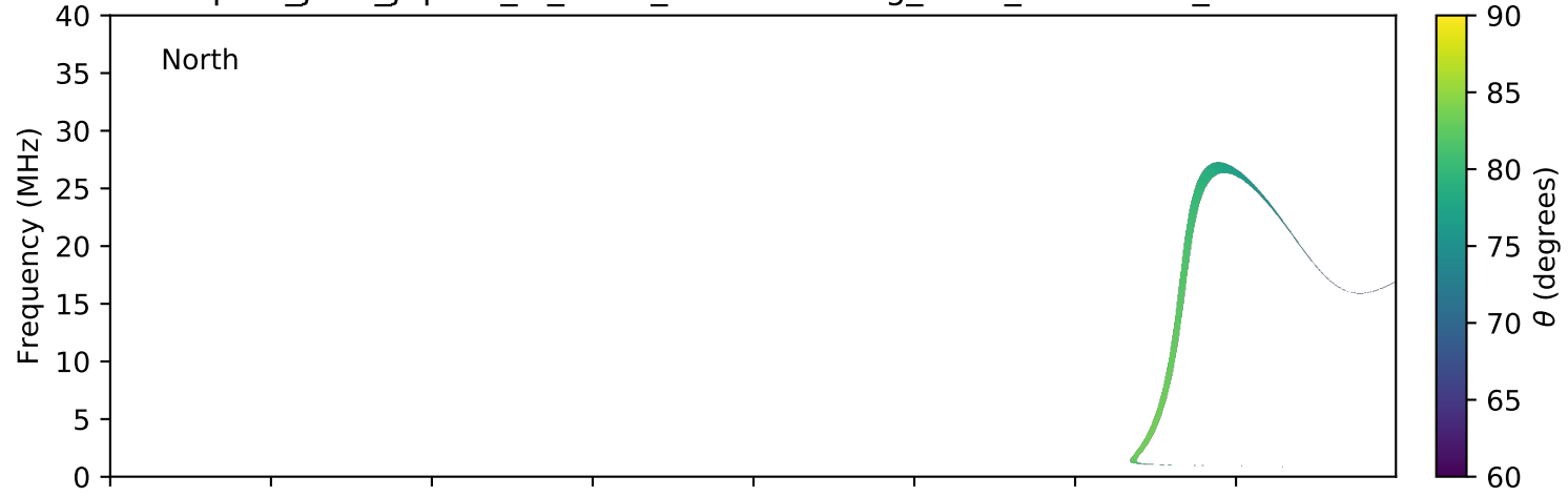
expres_juno_jupiter_io_isaac_lossc-wid1deg_3kev_20180501_v01.cdf
