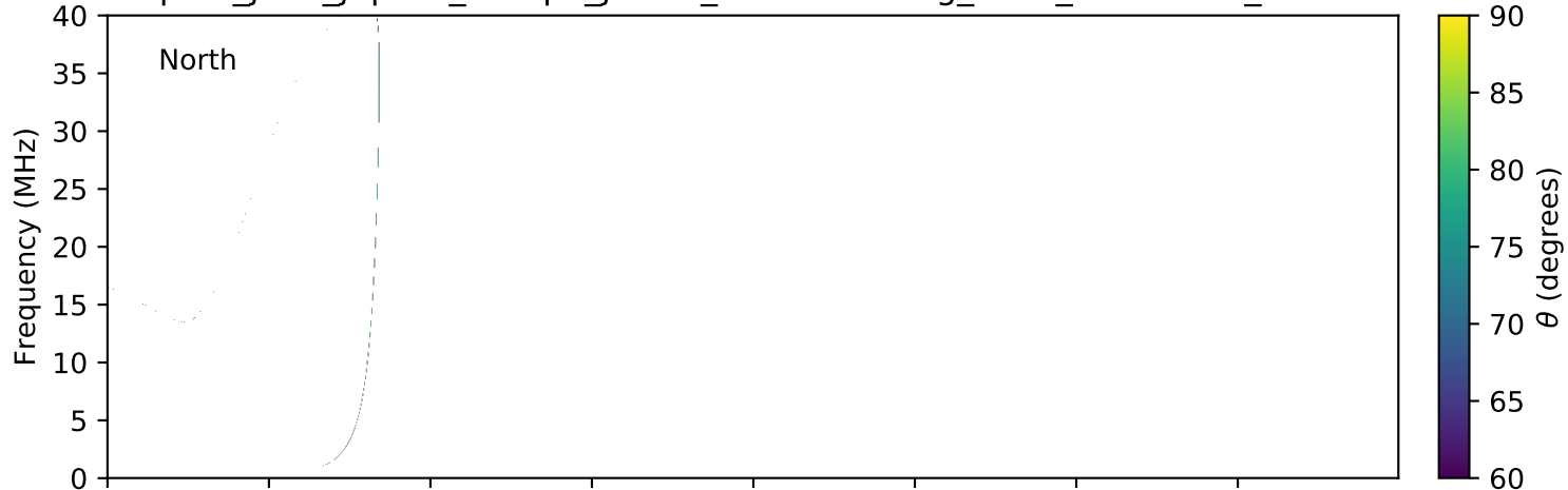
expres_juno_jupiter_europa_jrm09_lossc-wid1deg_3kev_20180524_v01.cdf
