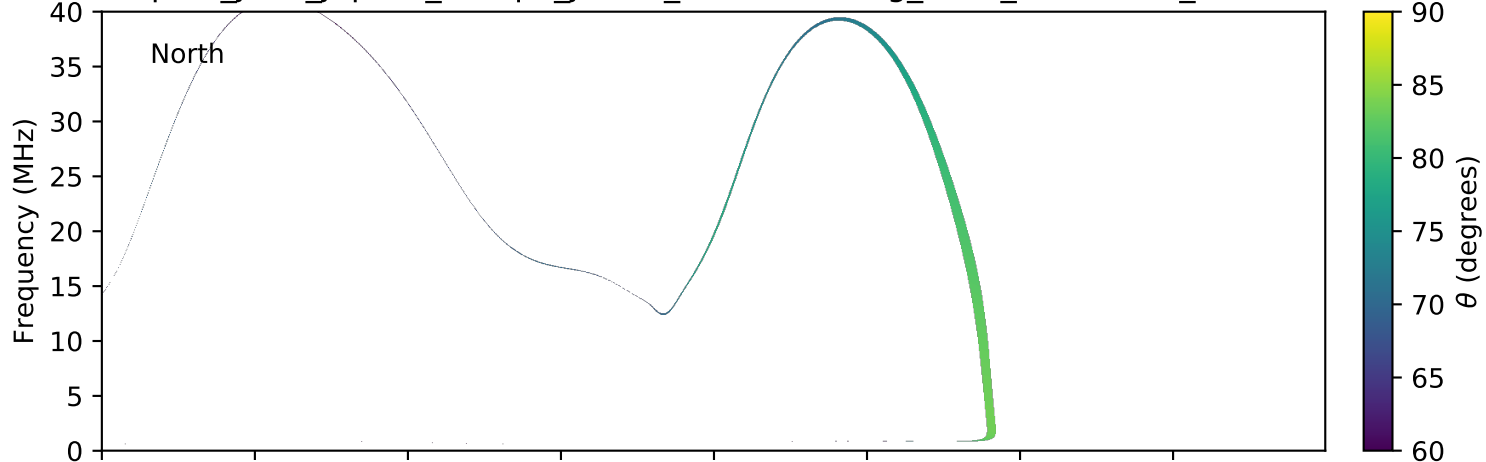
expres_juno_jupiter_europa_jrm09_lossc-wid1deg_3kev_20180522_v01.cdf
