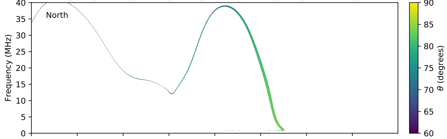
expres_juno_jupiter_europa_jrm09_lossc-wid1deg_3kev_20180520_v01.cdf
