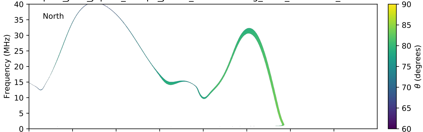
expres_juno_jupiter_europa_jrm09_lossc-wid1deg_3kev_20180517_v01.cdf
