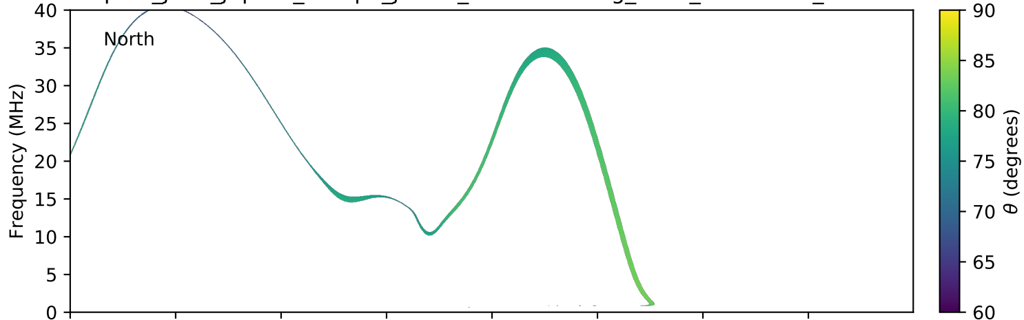
expres_juno_jupiter_europa_jrm09_lossc-wid1deg_3kev_20180515_v01.cdf
