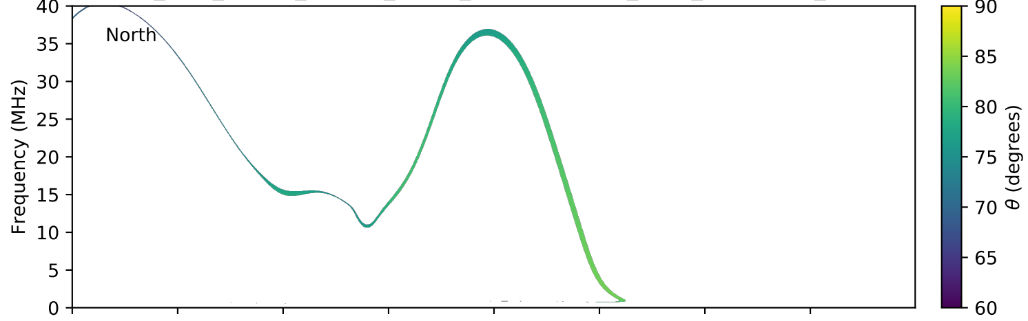
expres_juno_jupiter_europa_jrm09_lossc-wid1deg_3kev_20180513_v01.cdf
