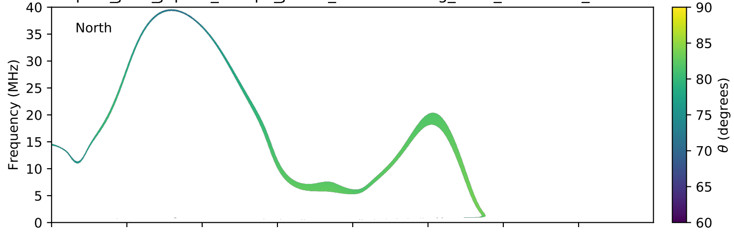
expres_juno_jupiter_europa_jrm09_lossc-wid1deg_3kev_20180505_v01.cdf
