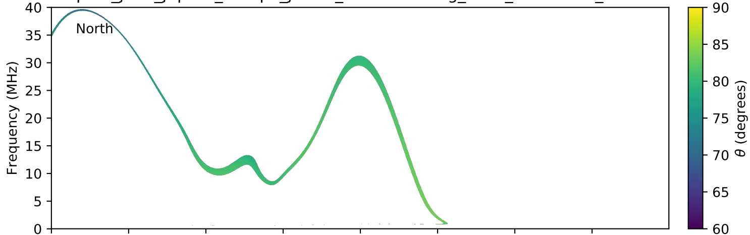
expres_juno_jupiter_europa_jrm09_lossc-wid1deg_3kev_20180501_v01.cdf
