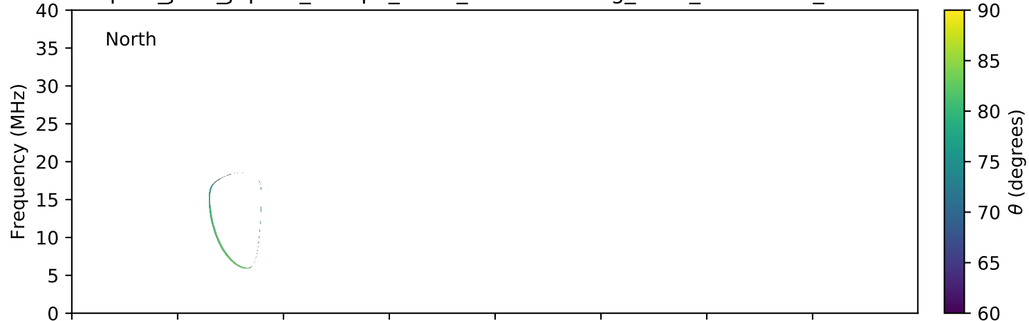
expres_juno_jupiter_europa_isaac_lossc-wid1deg_3kev_20180524_v01.cdf
