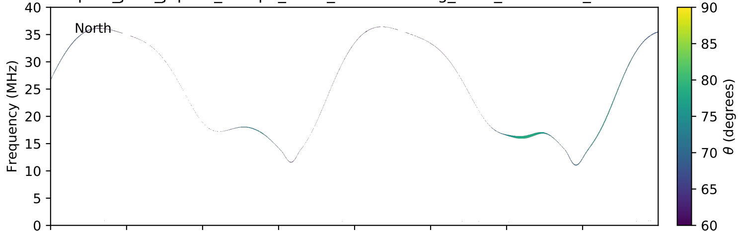
expres_juno_jupiter_europa_isaac_lossc-wid1deg_3kev_20180522_v01.cdf
