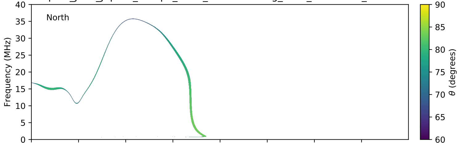
expres_juno_jupiter_europa_isaac_lossc-wid1deg_3kev_20180519_v01.cdf
