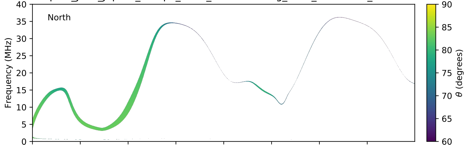
expres_juno_jupiter_europa_isaac_lossc-wid1deg_3kev_20180518_v01.cdf
