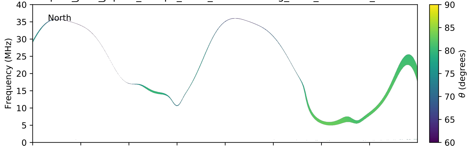
expres_juno_jupiter_europa_isaac_lossc-wid1deg_3kev_20180515_v01.cdf
