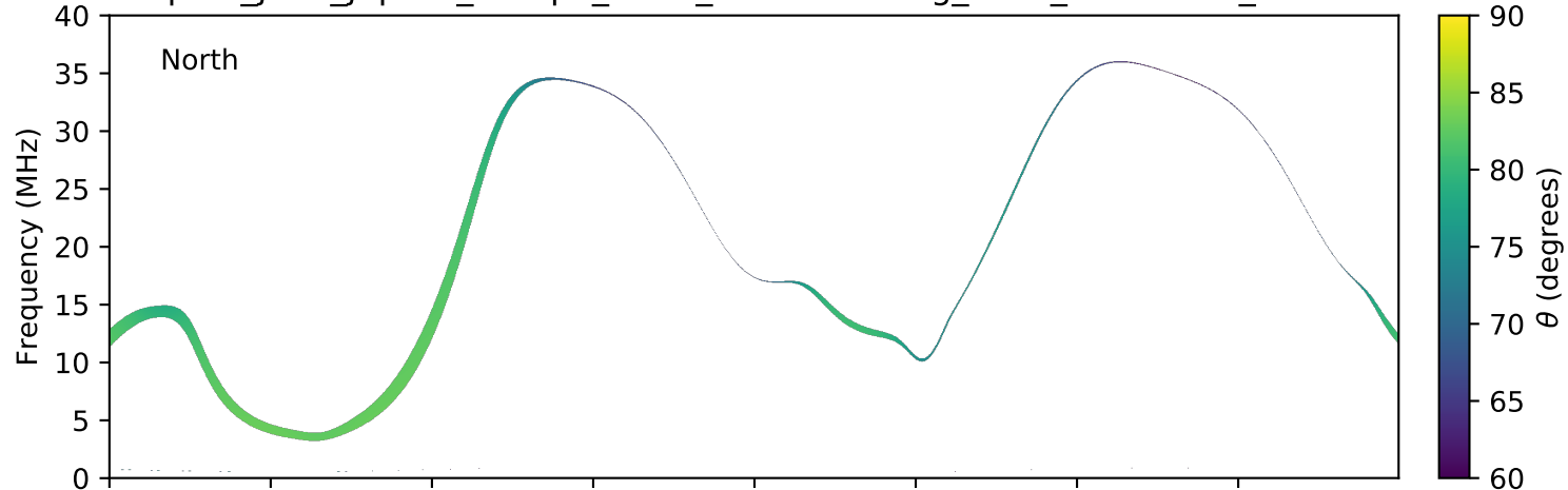
expres_juno_jupiter_europa_isaac_lossc-wid1deg_3kev_20180511_v01.cdf
