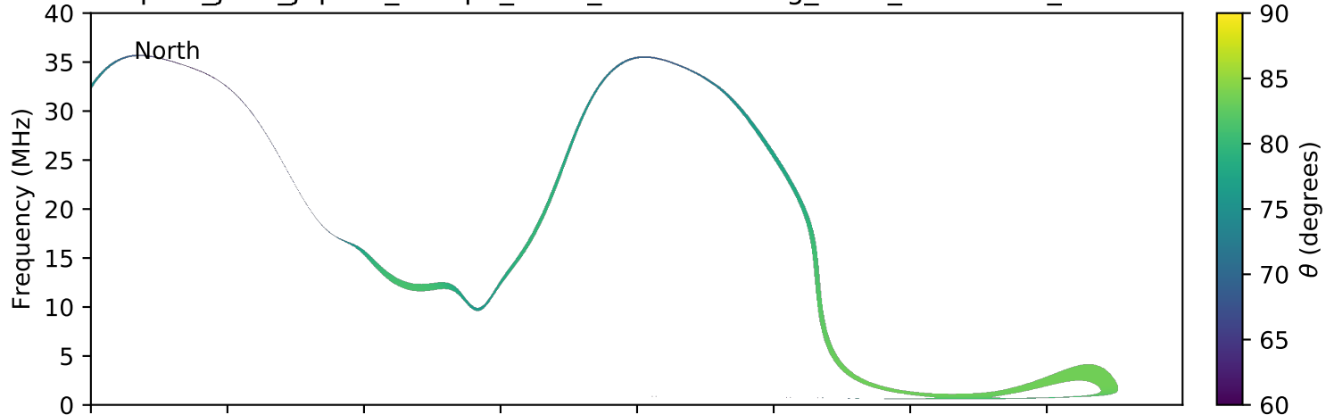
expres_juno_jupiter_europa_isaac_lossc-wid1deg_3kev_20180508_v01.cdf
