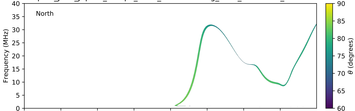
expres_juno_jupiter_europa_isaac_lossc-wid1deg_3kev_20180507_v01.cdf
